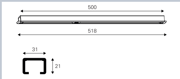
Mounting slide rail IS 21
