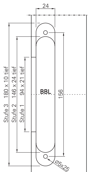
Milling drawing
